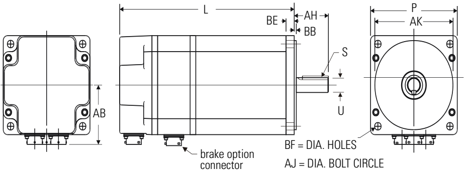
Figure 2 N-3400, N-4200, and N-5600 Mounting Dimensions
