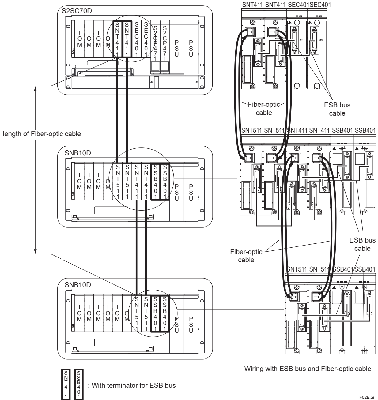
Figure Example of Chain Type Connection
