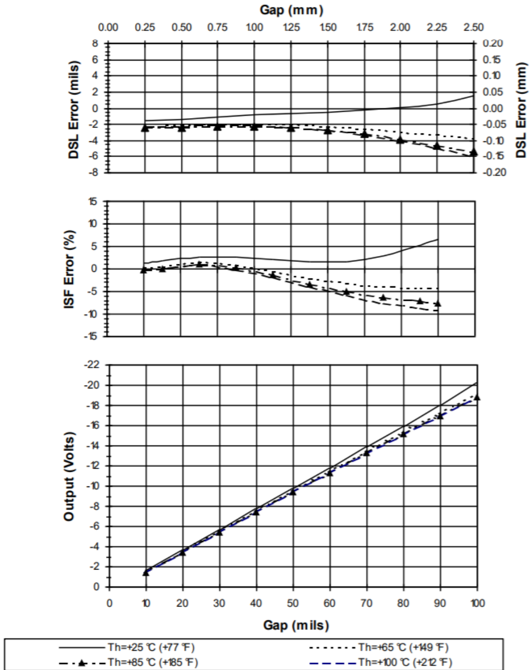
Figure 7: Typical 3300 XL 8mm 9m Proximitor Sensor with 8m Extension Cable at T_h (Probe is at 25 °C)
